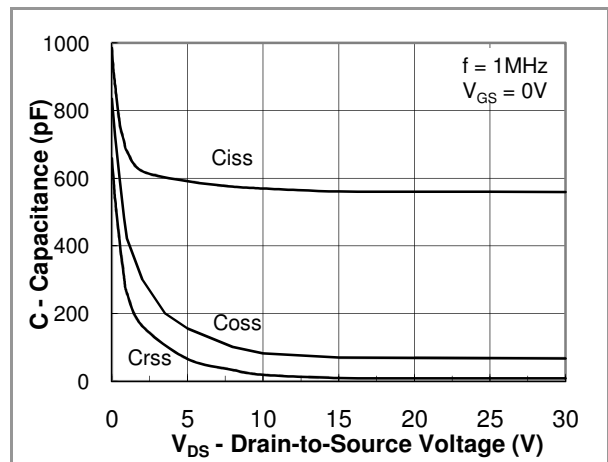
Fig.6 Capacitance
